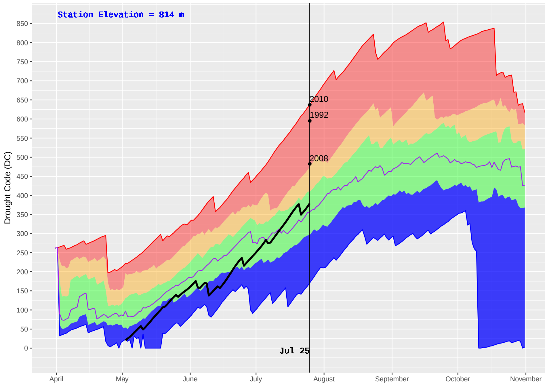
CHILAKO (189) : Historical (1986–2016) and Current (2018) Noon Drought Code (DC)
